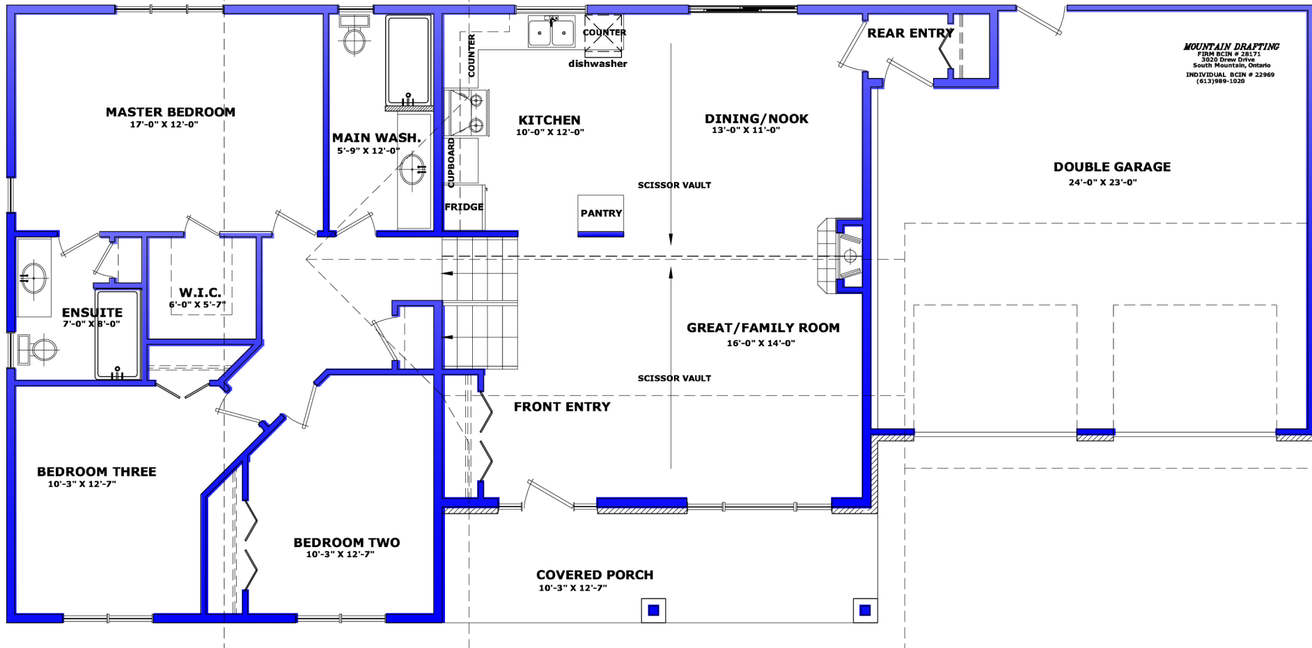
MODEL P2855 FLOOR PLANS 1492 SQFT
